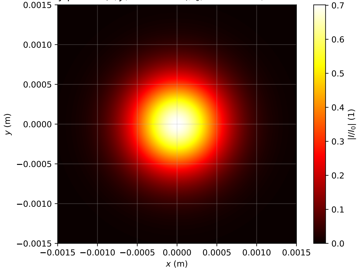
Intensity profile I(x, y, z = 1.831m)/I_0 , Pin=0.3Pcr, artificial time
